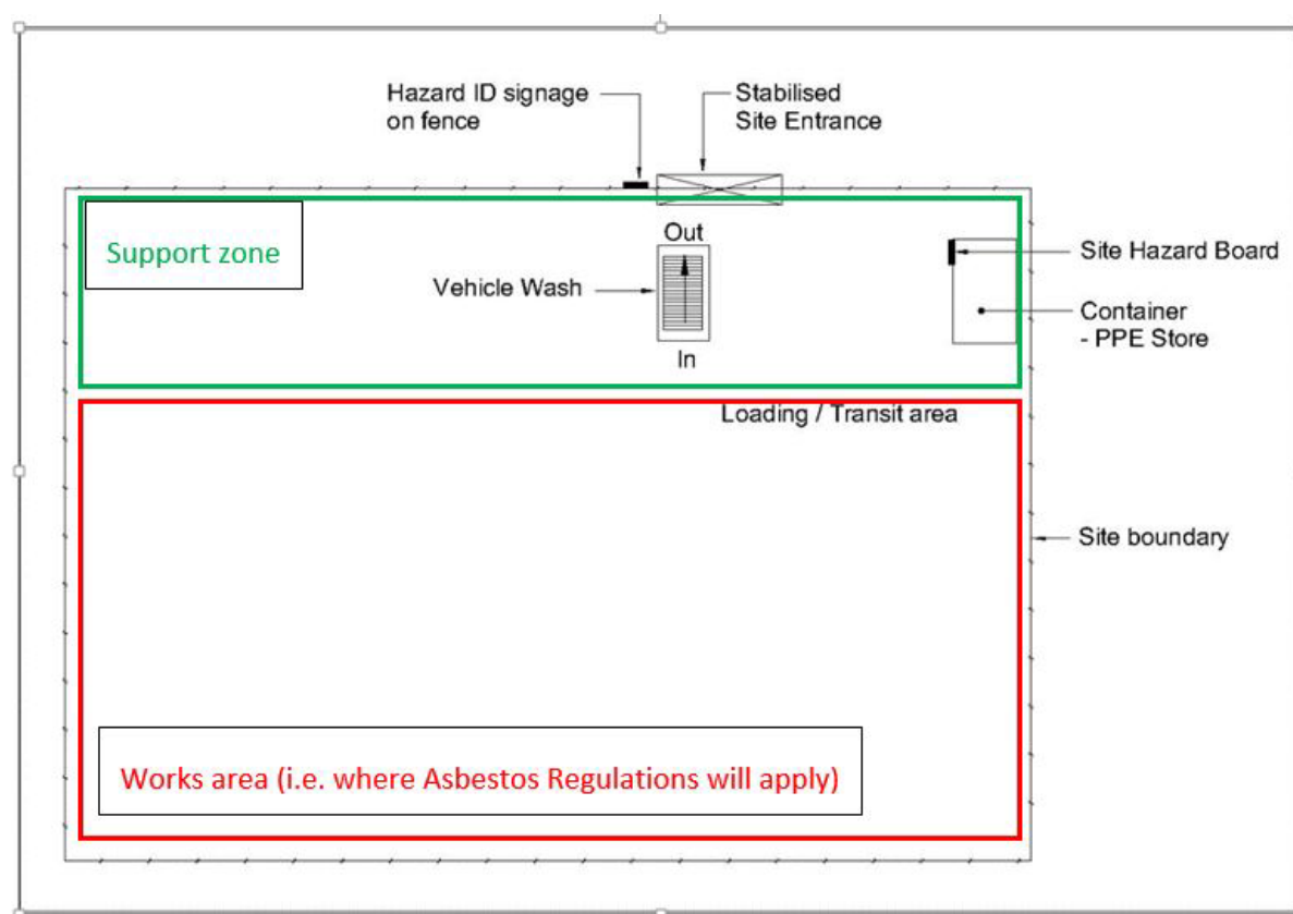
Figure 2.1: Indicative site establishment layout
